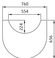
Contura 620/620T/690T Style, Glas Transparent Svart screenprint Dikte 6 mm
