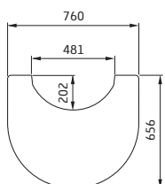
Contura 610/690 Style, Glas Transparent Svart screenprint Dikte 6 mm
